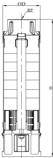
DIMENSIONS & WEIGHT
