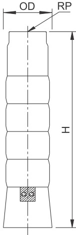
DIMENSIONS & WEIGHT
