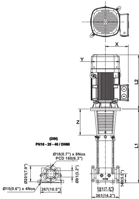
MVC (ROUND FLANGE)
