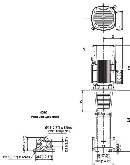
MVS & N (ROUND FLANGE)
