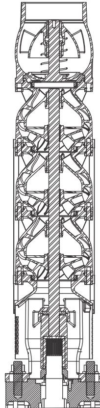
(10" & 8" Pump with 10" Motor - Spline)
