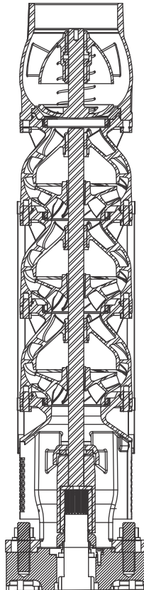
(8" & 10" Pump with 8" Motor)
