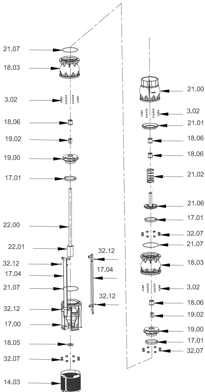
S8ST, S8NT, S10ST & S10NT
