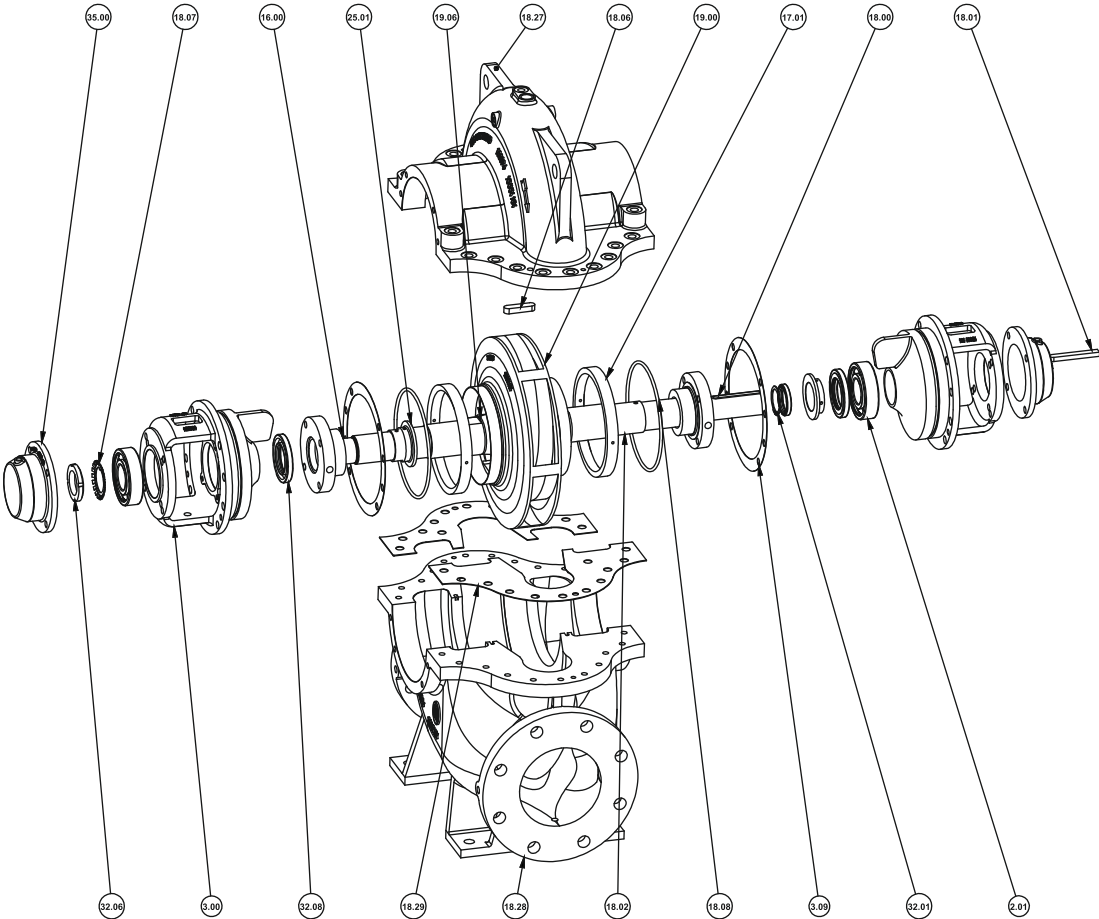
Exploded View
