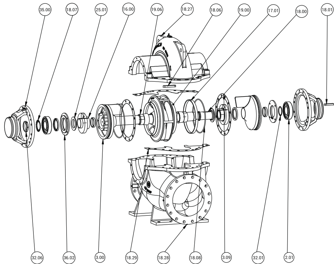
Exploded View
